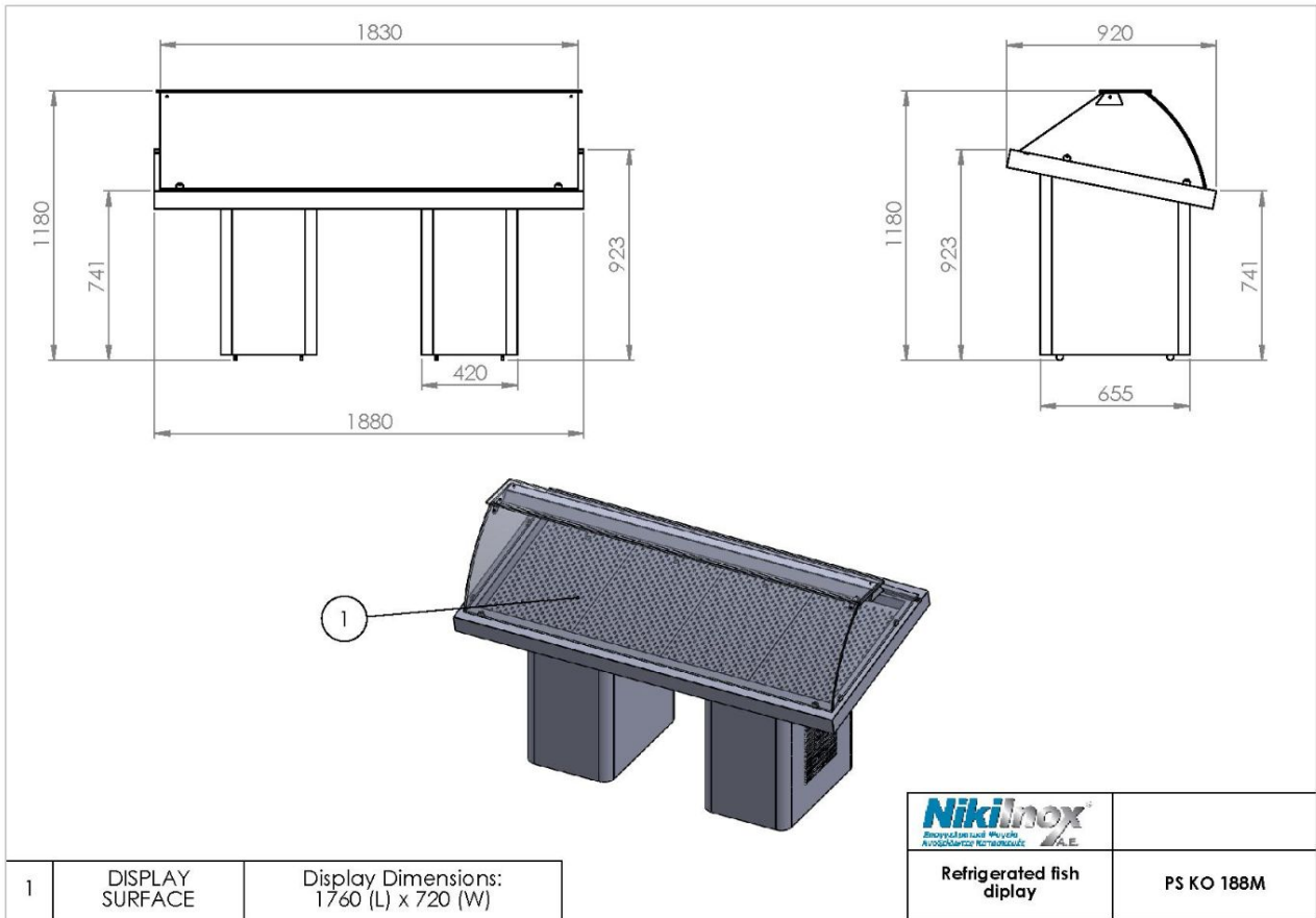
Technical Drawing
